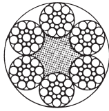
6 x 19 Seale (1+9+9) + FE
