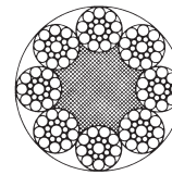
8 x 19 Seale (1+9+9) + FE
